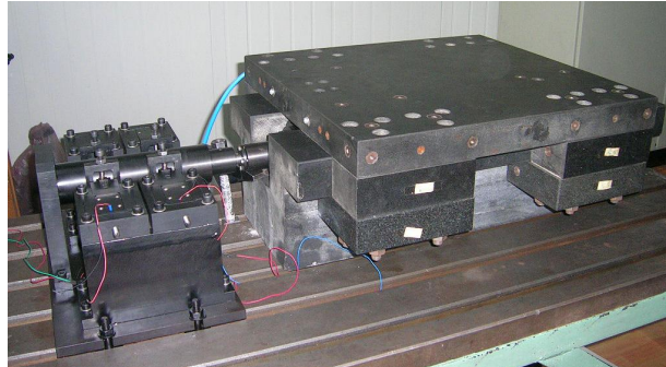
Figure 1: (b) Picture of the feed mechanism
