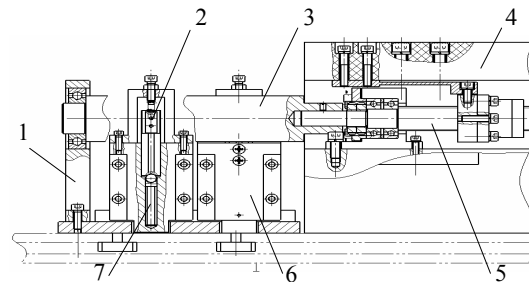
1-Bearing bracket 2-Friction gearing block 3 Friction gearing sleeve 4-Static-pressure air-bearing guide way 5- Ball screw 6- Piezoelectricity ceramic base 7-Piezoelectricity ceramic used for feeding
