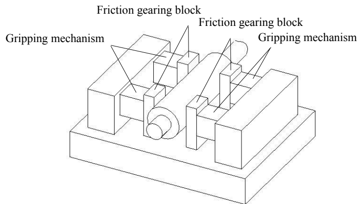
Figure 1: (b) Picture of the feed mechanism
