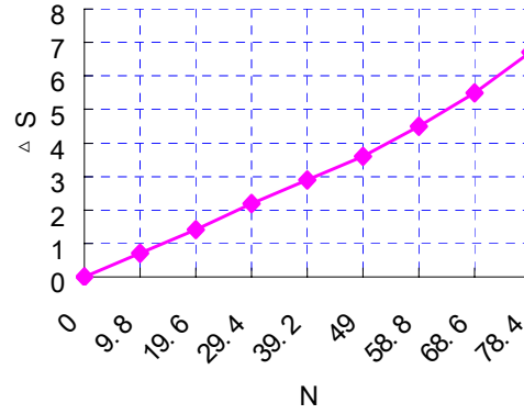
Figure 4: Rigidity curve of piezoelectricity ceramic
