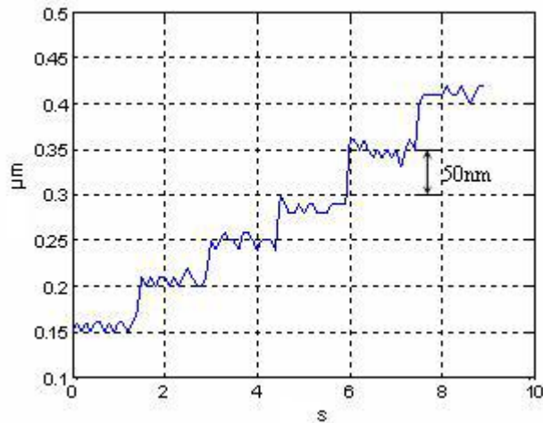
Figure 7: Distance resolution curve of feed mechanism
