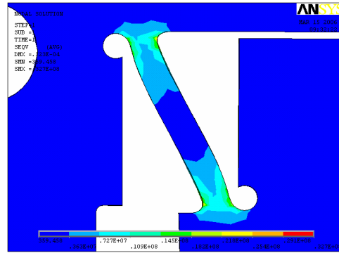
(c) Von-mises stress envelope
