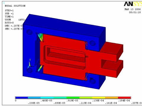
(b) Node motion nephogram
