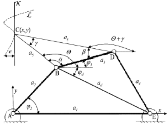
Fig. 3 Trajectory \mathcal{L} of the point C
