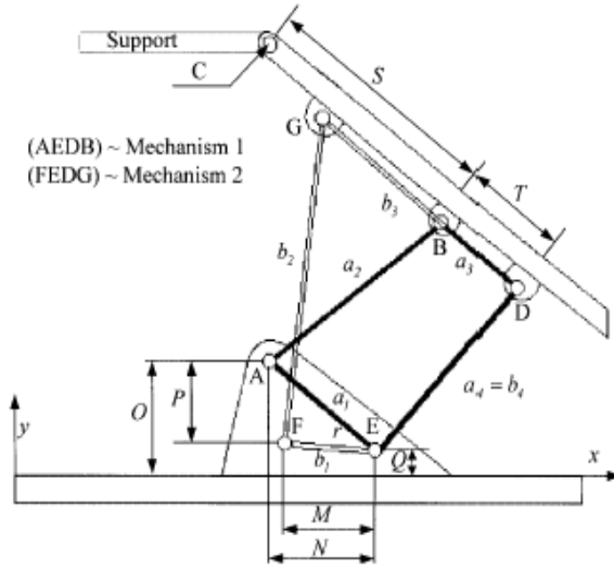
Fig. 2 Two four-bar mechanisms
