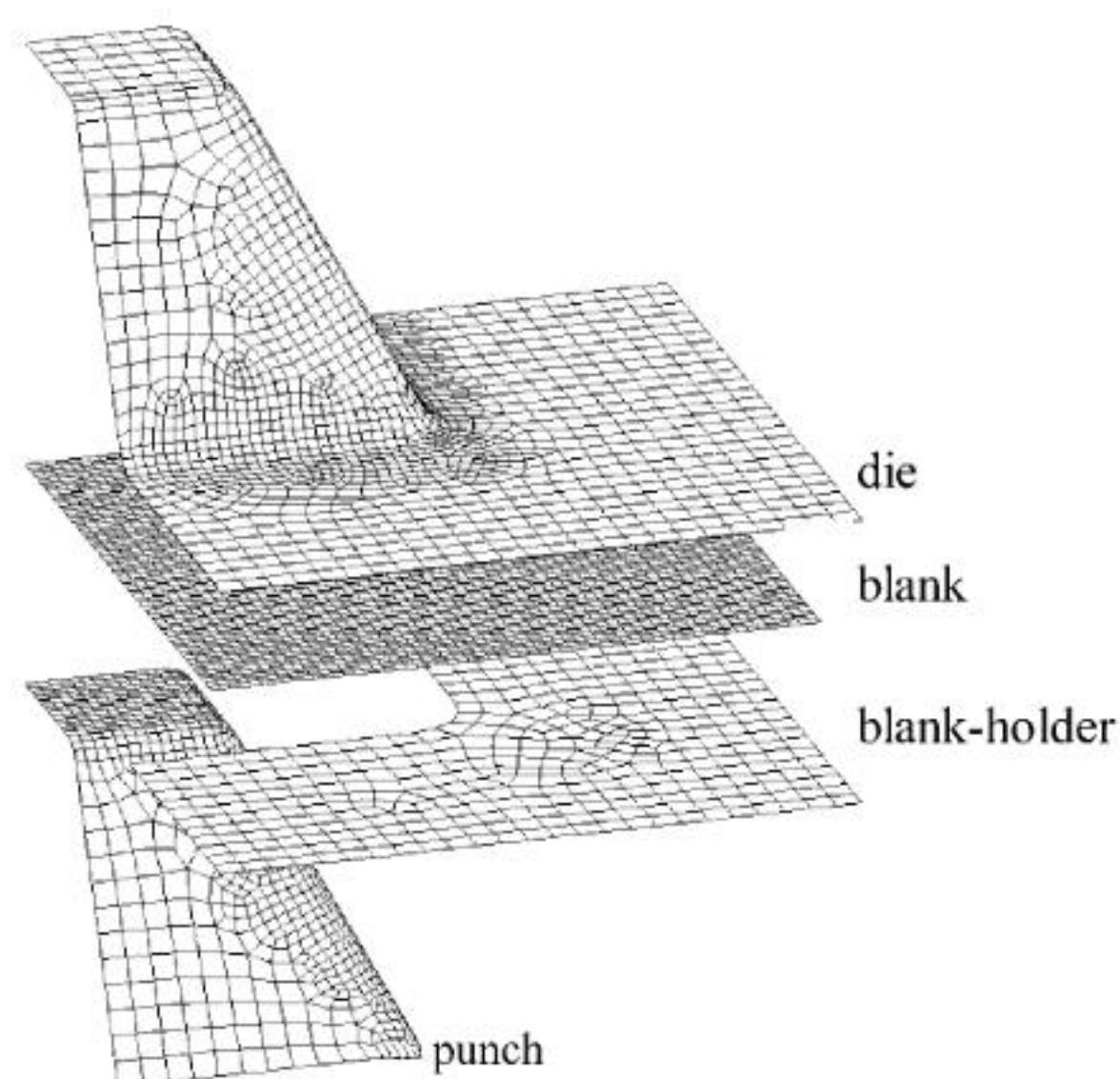
Fig. 2. Finite-element mesh.
