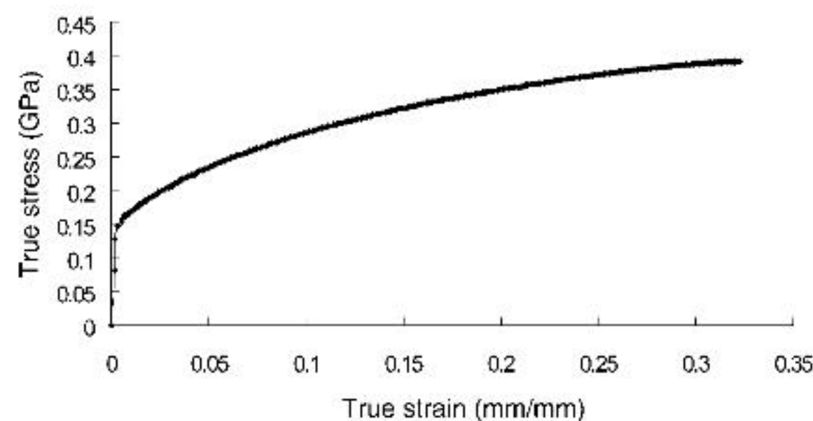
Fig. 3. The stress-strain relationship for the sheet metal.
