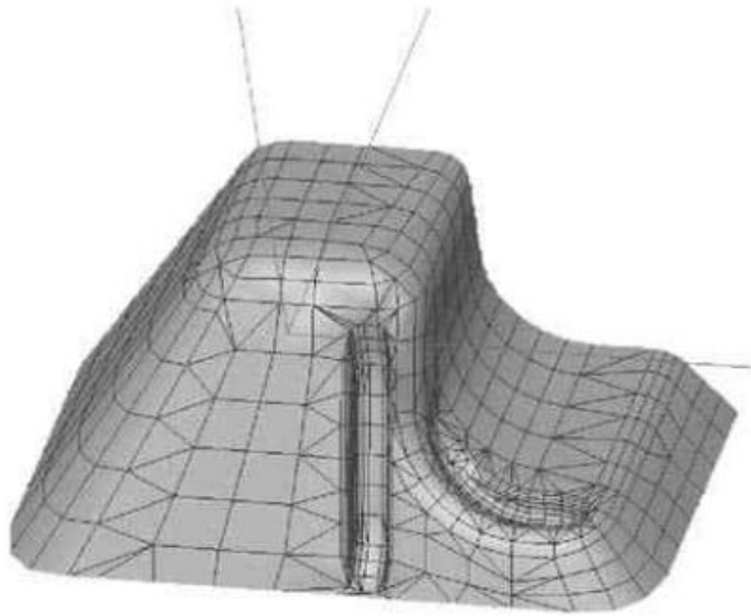
Fig. 9. Drawbars added to the draw walls.
