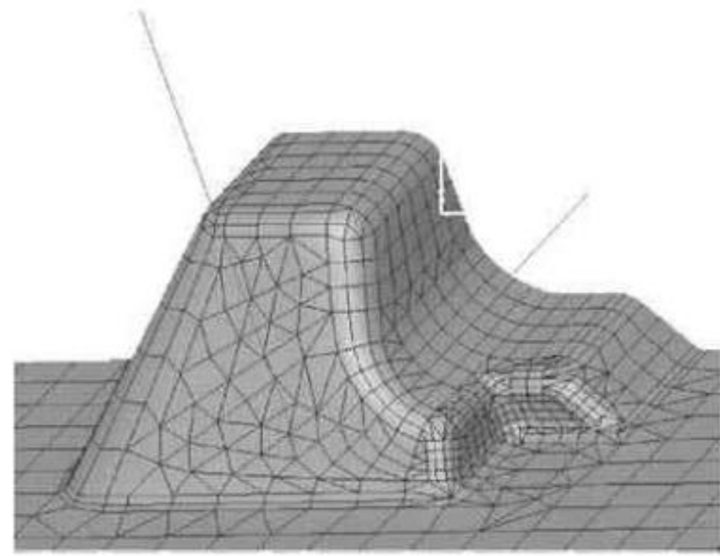
Fig. 11. Cut-off of the stepped corner.
