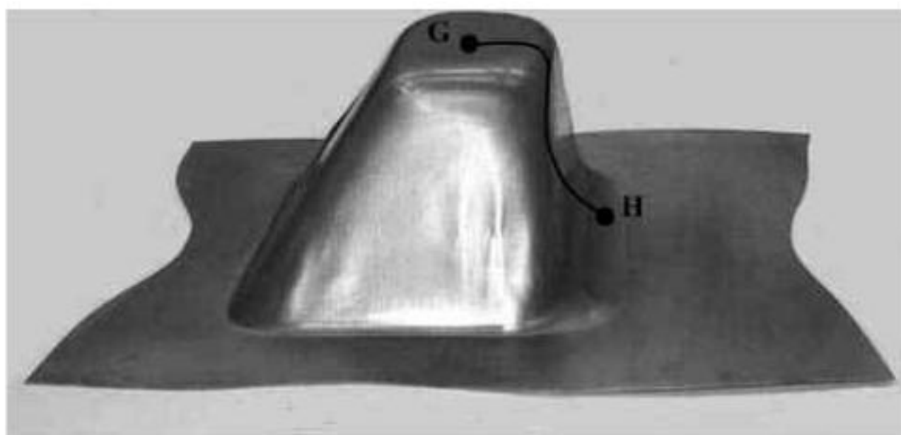
Fig. 14. The defect-free production part.
