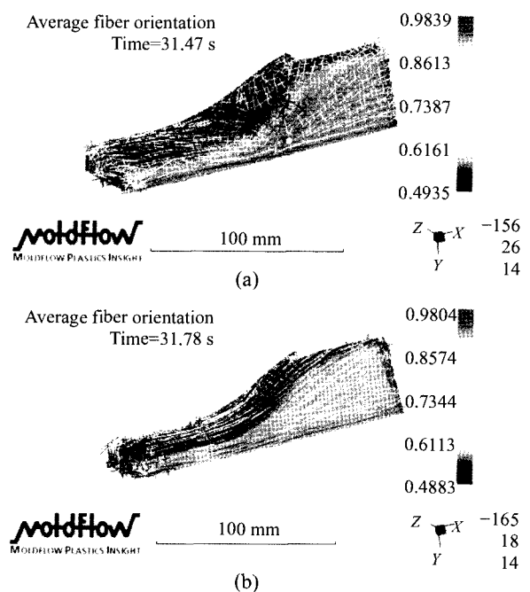
Fig.6 The orientation distribution of the glass fiber with varied gate location
