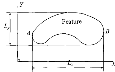
Fig.2 The projected length evaluation
