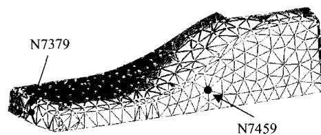
Fig.5 Finite element mesh model of the part
