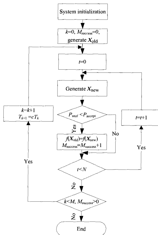
Fig.3 The flow chart of the simulated annealing algorithm
