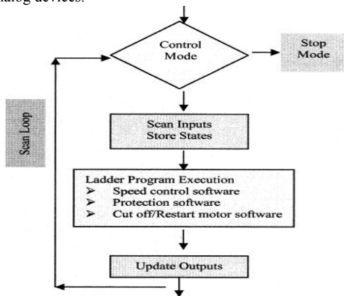
Fig. 3. Flowchart of the main program.
