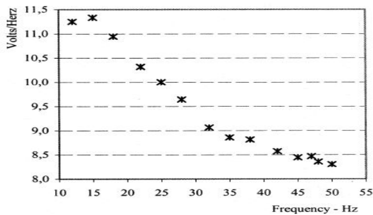
Fig. 10. Rate for stator voltage/stator frequency.
