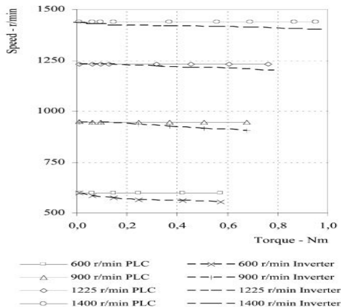
7. Experimental speed–torque characteristics with PLC and inverter.
