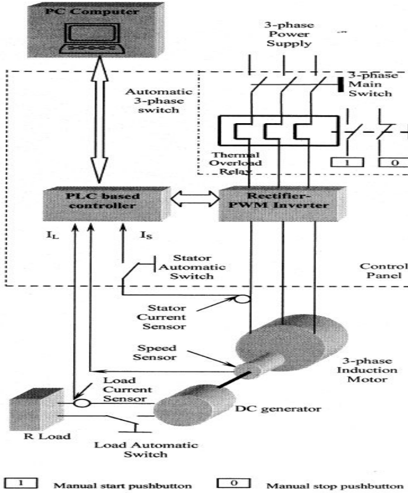
Fig. 2. Electrical diagram of experimental system.
