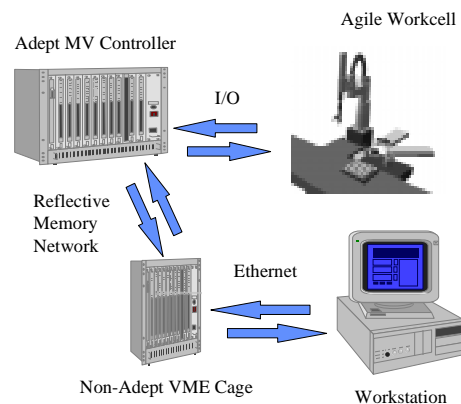
Figure 4: System Architecture
