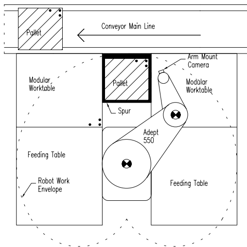
Figure 2: Workstation Layout
