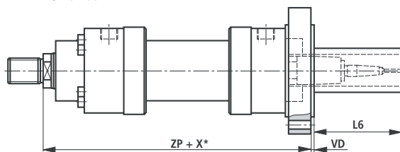
MF4: AL-Ø 40 - 63 mm
