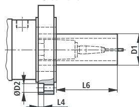
MF4: AL-Ø 80 - 320 mm
