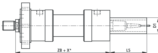
MF4: AL-Ø 80 - 320 mm
